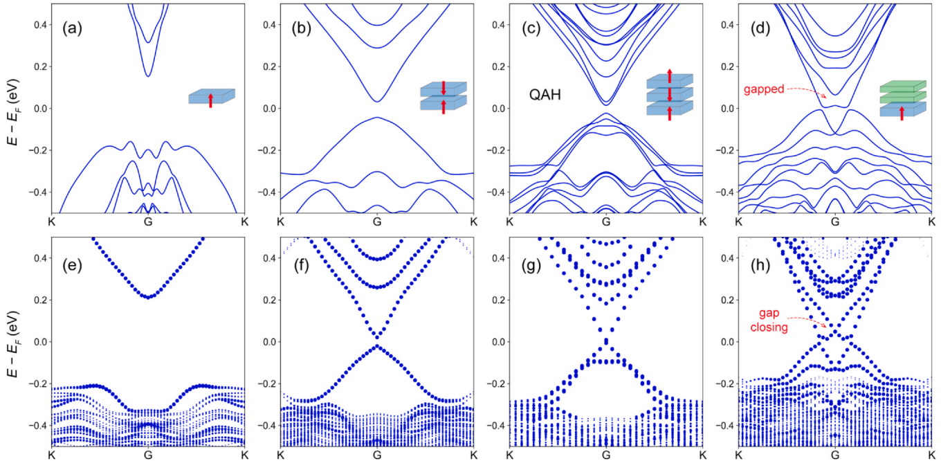
Fig. 3. (a–d) Calculated band structures of the thin film 1 SL, 2 SL, 3 SL, and SL-2QL, respectively. The AFM ground state is assumed. The 3 SL is a QAH insulator. (e–h) Band structures in the PM phase. Spectral weights are shown as the size of blue dots.
