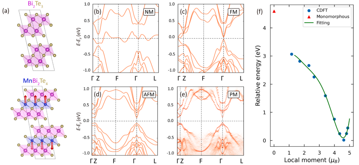
Fig. 2. (a) Crystal structure of \text{Bi}_2\text{Te}_3 and \text{MnBi}_2\text{Te}_4 with an A-type AFM configuration. (b)–(d) Band dispersions of the (b) NM, (c) FM, and (d) AFM configurations. For the calculations of NM and FM phases, we use a single SL which causes double Brillouin zone length along \Gamma –Z. (e) The spectral functions of the PM phase by the polymorphous description with randomly distributed local moments. The spin-orbit coupling is included. (f) Total energy as a function of constrained local moments with an AFM configuration. A polynomial function is used to fit the total energy evolution.
