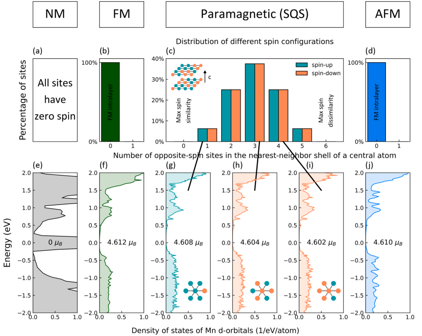
Fig. 1. The spin configuration and corresponding projected local density of states (PDOS) in \text{MnBi}_2\text{Te}_4 . (a)–(d) Upper panel: The weight of local spin configuration F(n^{\uparrow\downarrow}) in different spin configurations. (a) All the metal sites are identical for zero spins. (b) and (d) The spins of nearest neighbor cations in a layer, keep the same direction in the FM and A-type AFM phases ( n^{\uparrow\downarrow} = 0 everywhere). (c) Distribution of the weights of local spin configurations in the PM supercell modeled by the 224-atom SQS shown in the inset (only the Manganese sites are shown). The bars describe the percentage of nearby opposite-spin sites when the central atom is spin-up (green) and spin-down (coral). (e)–(j) Lower panel: The d -orbitals PDOS of the manganese atom in the upper panel, respectively. (e) The NM model with a single atom in a unit cell induces a metallic gapless phase. (g)–(i) In the PM-SQS structure, the magnitude of moments in different local environments varies in a small range, and there is no accidental band gap closure for each individual atom. The inset shows the central atom's environment corresponding to n^\uparrow = 5, 3, 2 ( n^\downarrow = 1, 3, 4 ). (f) and (j) FM and AFM motifs.
